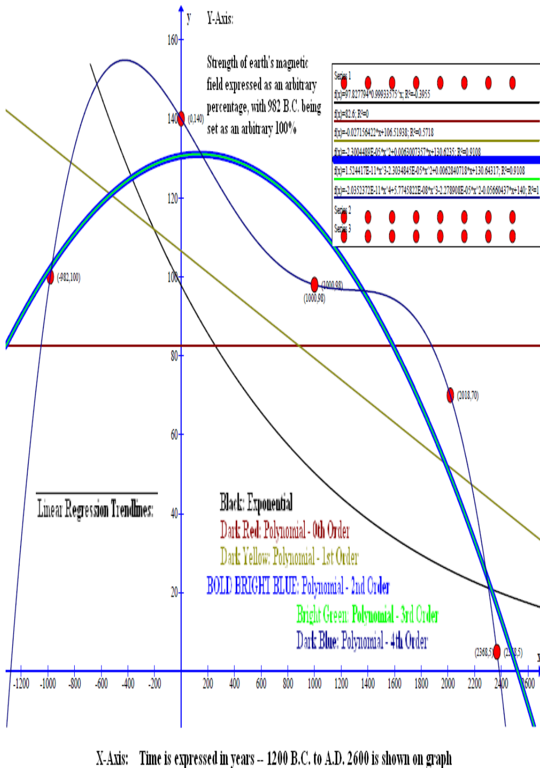
Image 10. "Linear Regression" GRAPH of changes in the dipole strength of earth's protective geomagnetic field, as a function of time. DATA used for this graph are the five (5) data points taken from Table 4. of this paper, and using "5%" for the 5th and last data point, where a choice is given.
