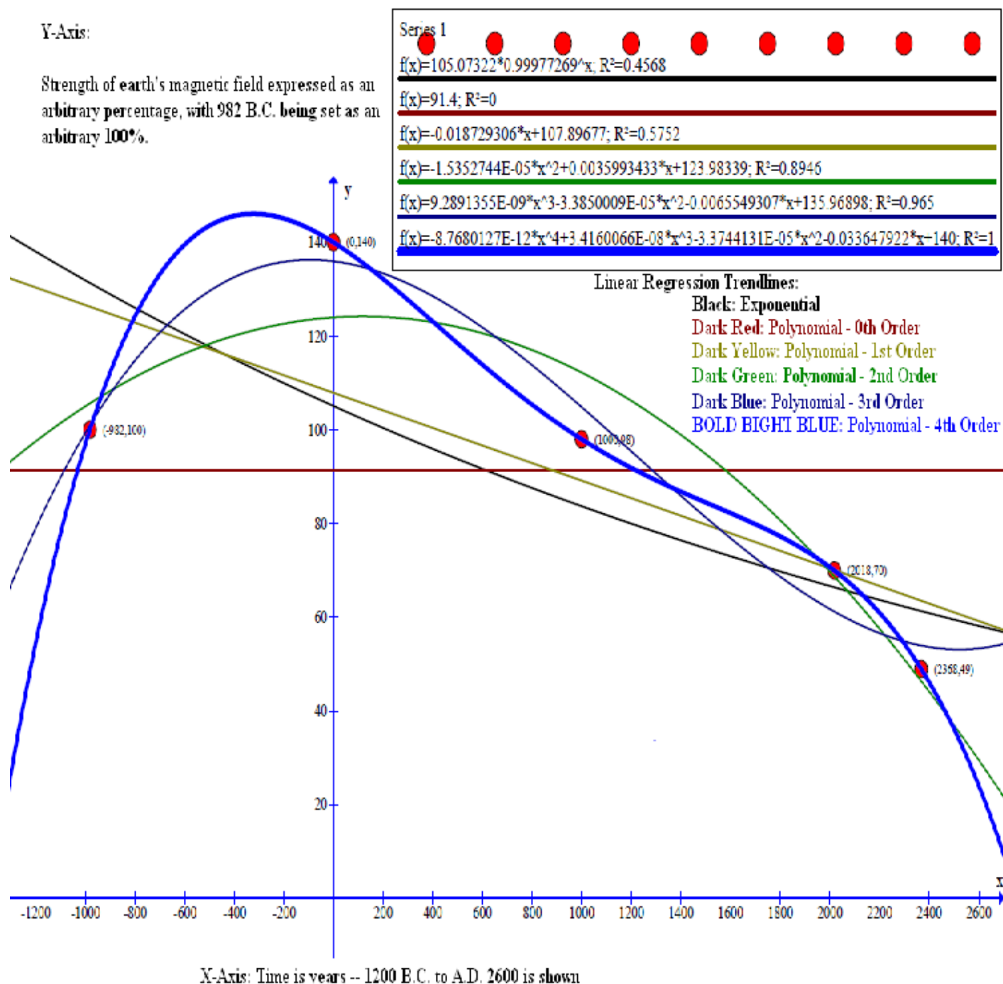
Image 9. "Linear Regression" GRAPH of changes in the dipole strength of earth's protective geomagnetic field, as a function of time. DATA used for this graph are the five (5) data points taken from Table 4. of this paper, and using "49%" for the 5 th and last data point, where a choice is given.
